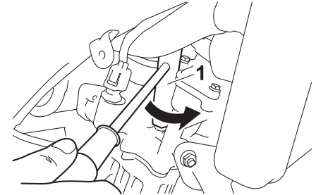
1. Zündkerzenschlüssel
