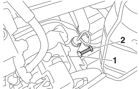
1. Locknut 2. Chain tension adjusting bolt
