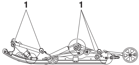
1. Grease nipple
