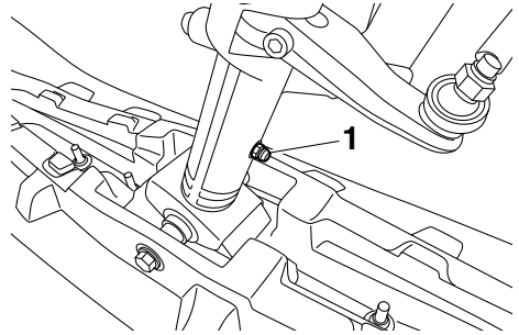
1. Grease nipple
