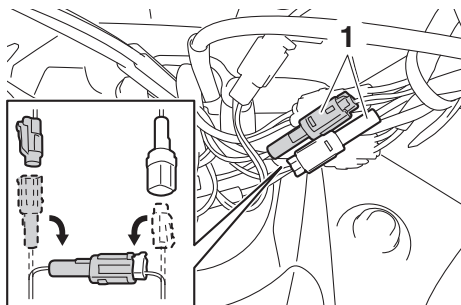
1. Throttle switch connector
