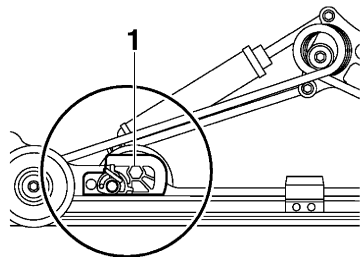
1. 2-up adjusting block
