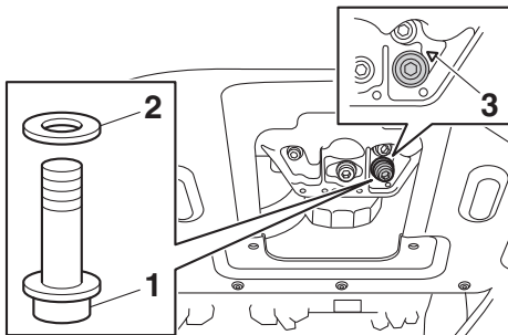
1. Engine oil drain bolt (crankcase) 2. Gasket 3. “▽” mark
