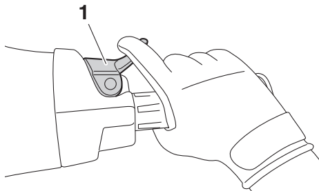
1 Throttle lever
