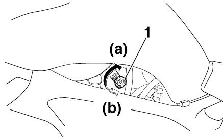
1. Stationair stelschroef
