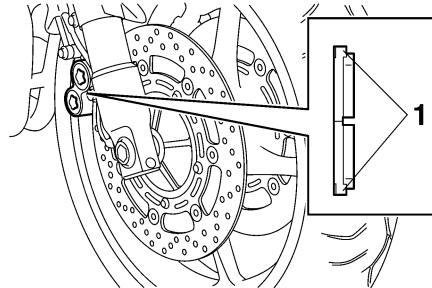
1. Slijtage-indicator remblok
