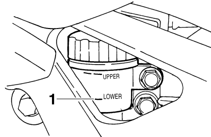
1. Merkstreep minimumniveau
