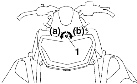
1. Headlight beam adjusting screw
