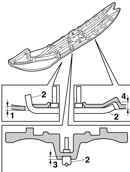
1. Ski runner wear limit
