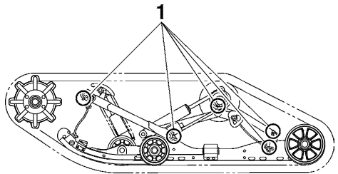
1. Grease nipple
