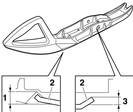
1. Ski runner wear limit
