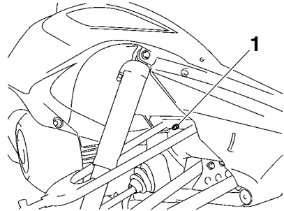
1. Grease nipple
