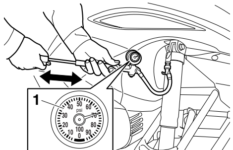
1. Pressure gauge (low-pressure meter)
