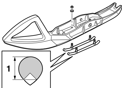
1. Ski runner wear limit
