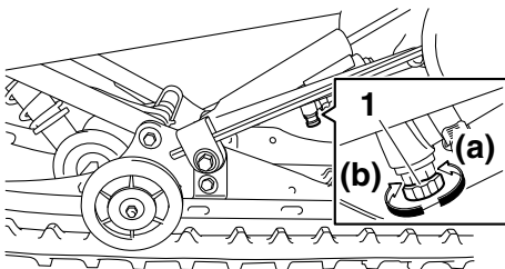
1. Compression damping force adjusting knob
