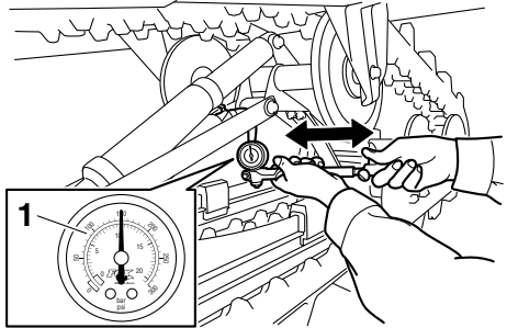
1. Pressure gauge (high-pressure meter)
